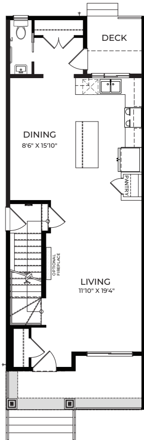
Main Floor ± 686 ft 2
